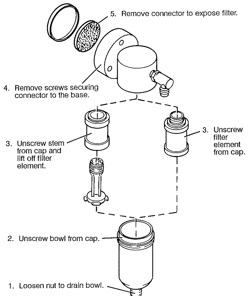
Figure 4-6. Disassembling the Gas Supply Water Trap and Filter Assembly (screw-type drain)
